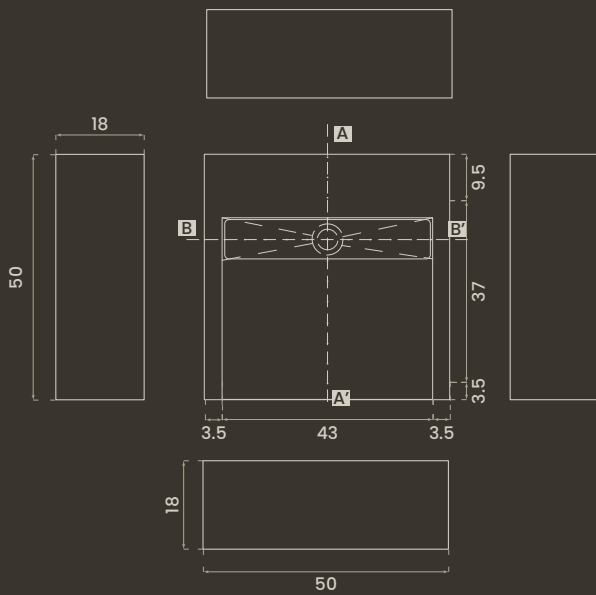
SENO RAMPA · INCLINED SINK
