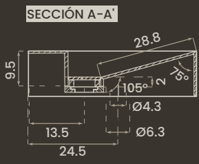
SENO RAMPA · INCLINED SINK
